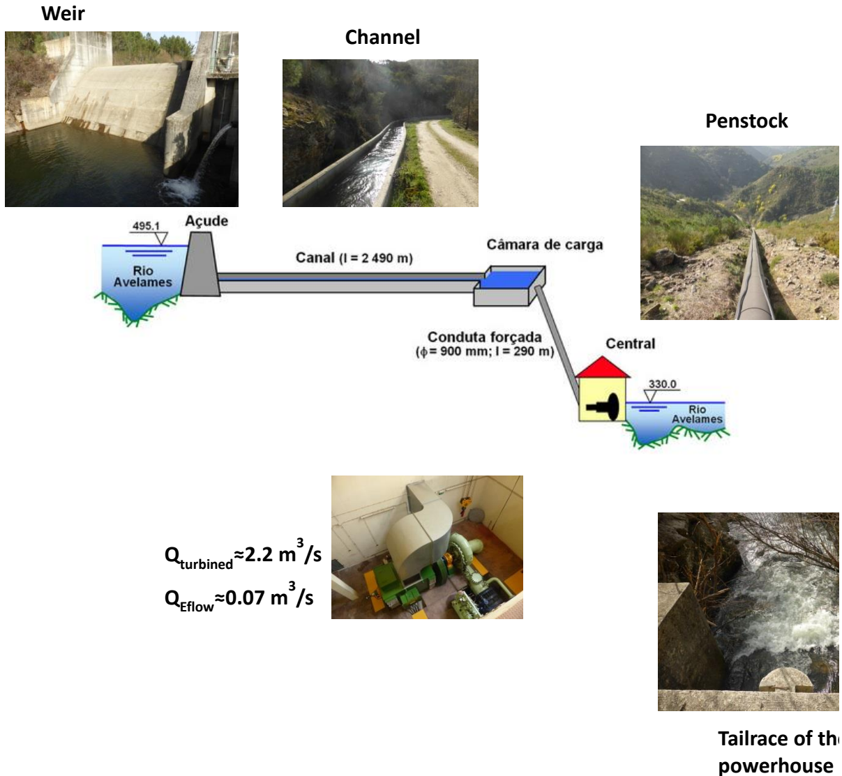
Figure 5 - Bragado HPP scheme
