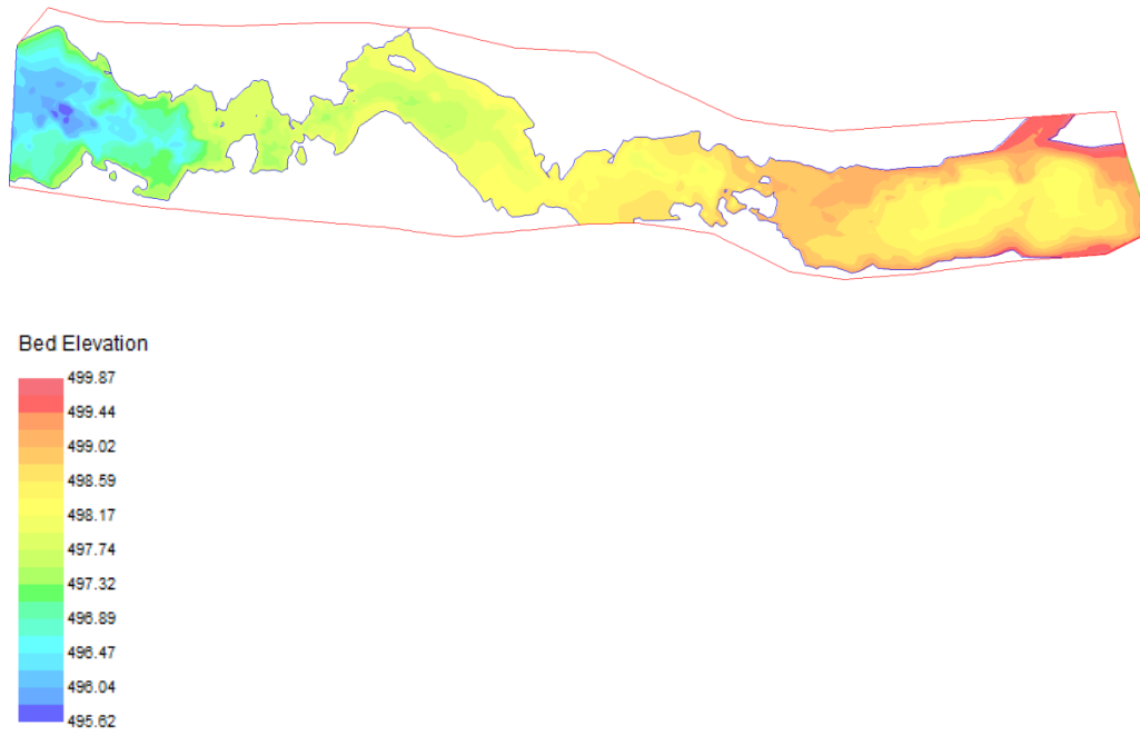
Figure 19 – River bed topography at the upstream river reach.
