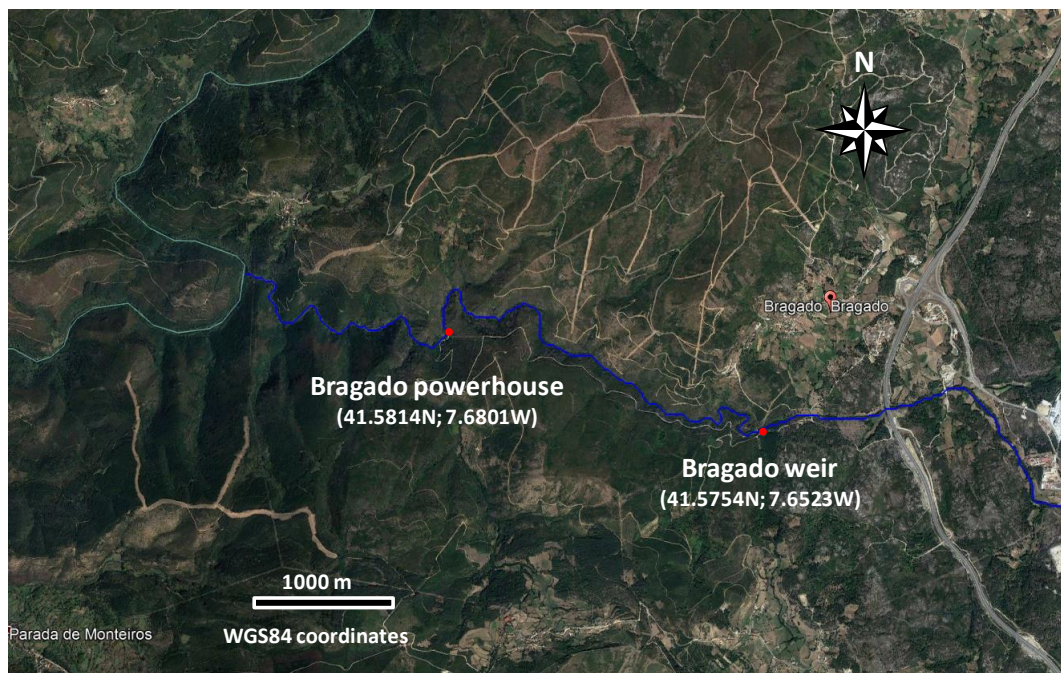
Figure 4 – Location of Bragado HPP and Bragado weir
