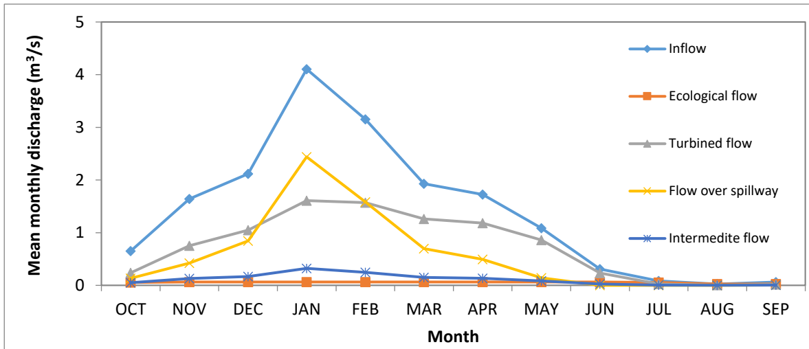
Figure 16 – Mean monthly flows at Bragado HPP scheme.
