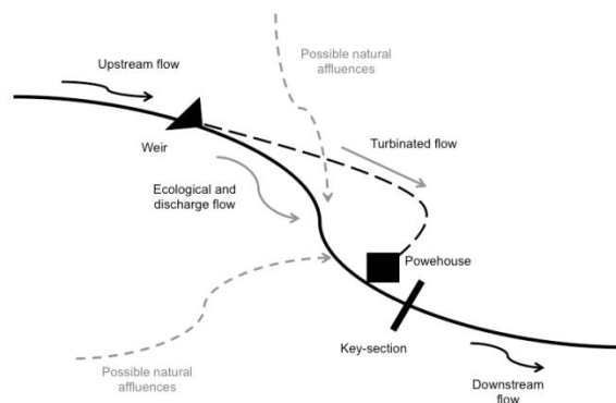
Figure 14 – Bragado HPP scheme. Localization of the weir, HPP and key-section.
