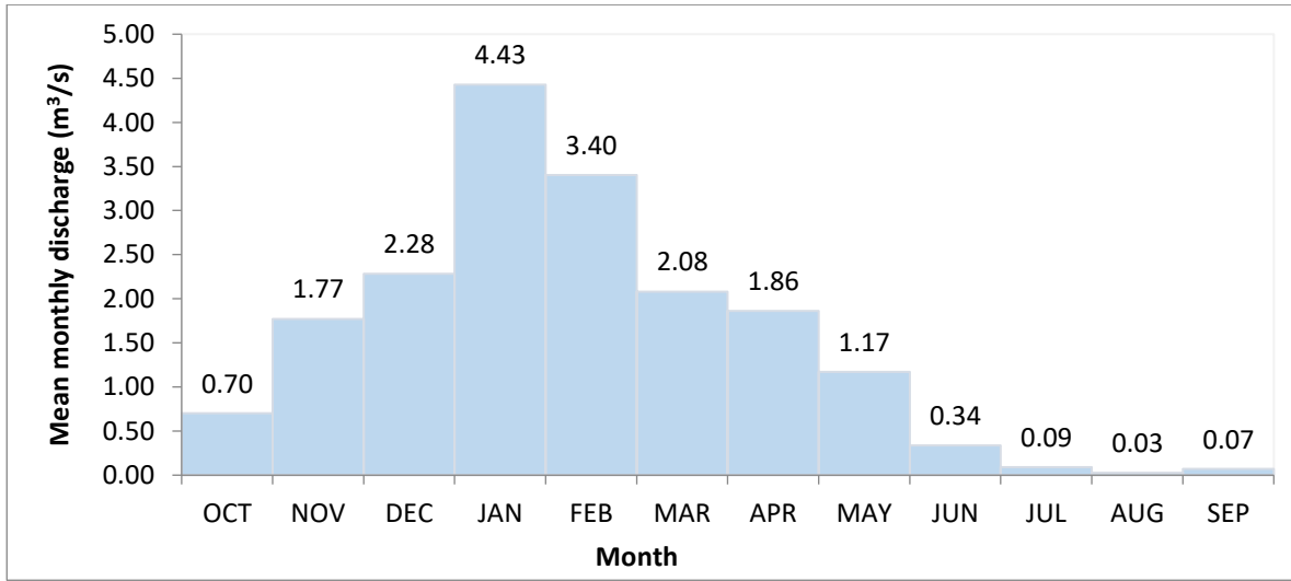
Figure 3 - Mean monthly discharge downstream Bragado HPP (2010-2016)
