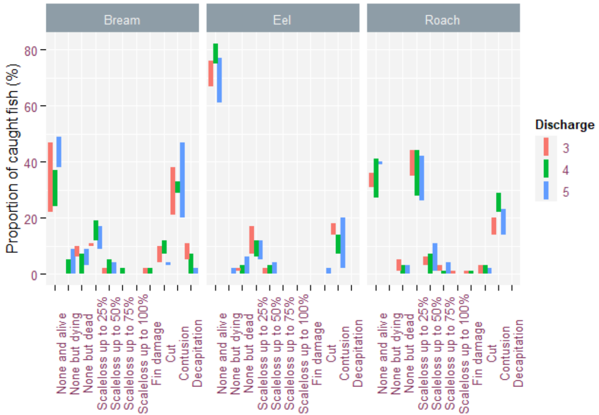
Figure 14 Proportions of caught fish per state (alive, dead or dying) and injury type for the three operational modes of the tested Archimedes type hydrodynamic screw: 3, 4 and 5 m 3 /s.
