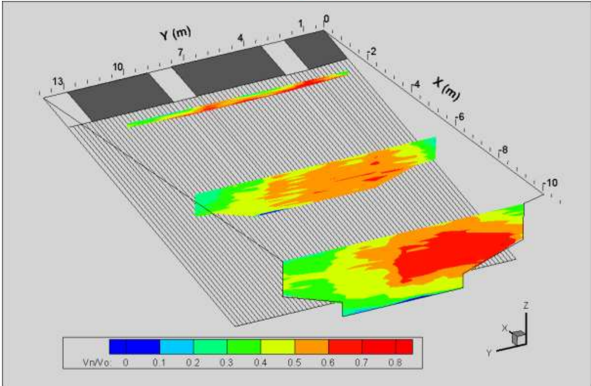
Figure 53: Cartographies of V_t/V_0 (up) and V_n/V_0 (down) measured at Las Rives, V_0=0.29 m/s, 2017.
