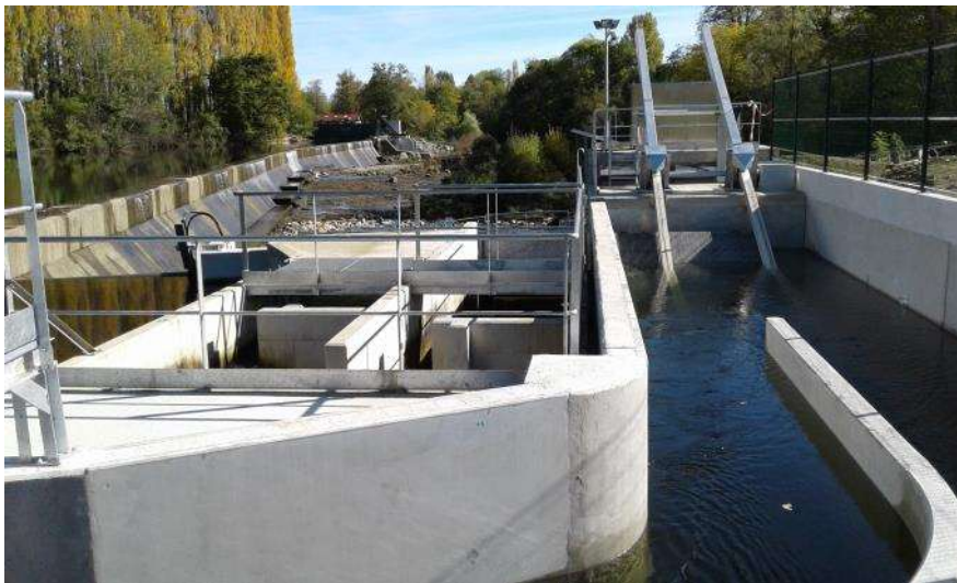
Figure 27: Fish pass and the new DIVE turbine on the bypassed reach
