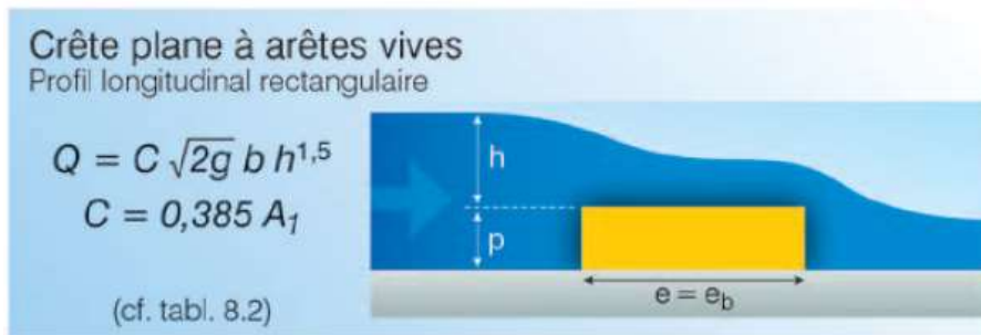
Figure 65: Expression of the discharge coefficient for a thick weir with a plane crest and sharp edges (source: (Le Coz, et al., 2011)).
