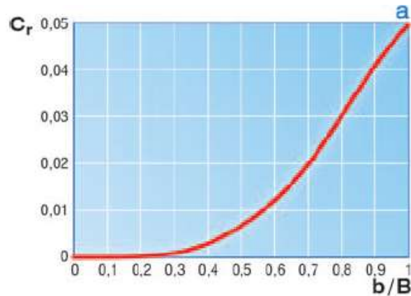
Figure 67: Abacus for the determination of C_r for a weir with thin wall and rectangular section (Le Coz, et al., 2011)
